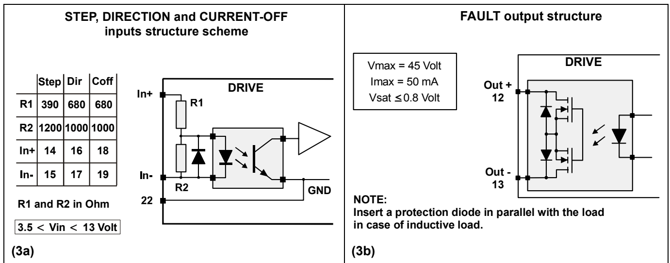
Fig. 3 – Inputs and outputs scheme.
